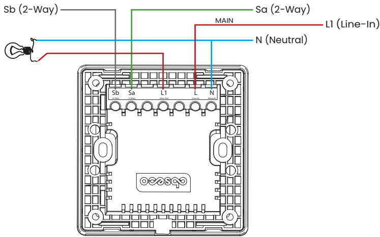
Figure 1: Wiring Diagram – 1-Way Installation
